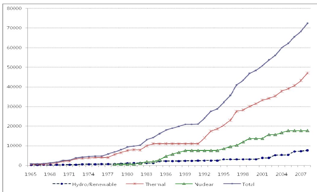
Figure A6: Installed Capacity of Electric Power by Fuel Source (MW)
